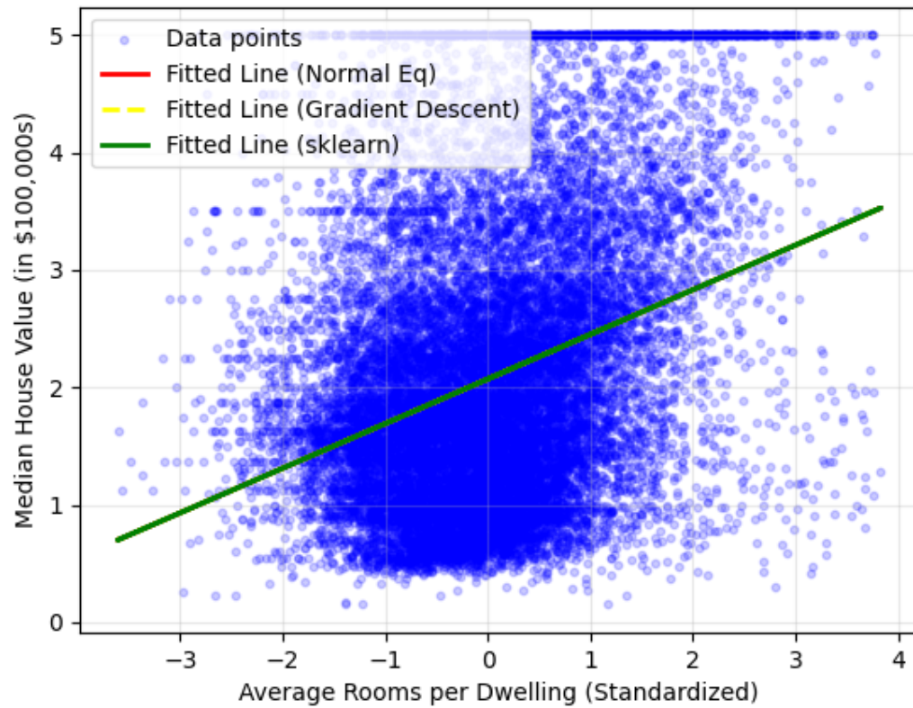
Linear Regression: California Housing (AveRooms vs Price)
