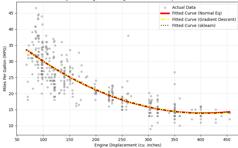
Polynomial Regression (Degree 2): MPG vs. Displacement
